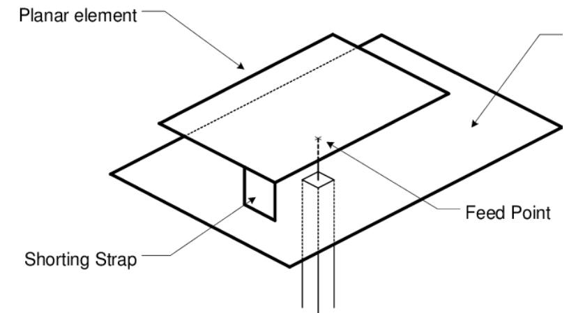
Figure: Planar inverted-F antenna
