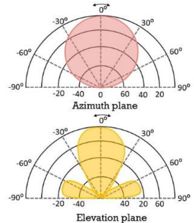
(a) Radiation pattern of Microstrip Antenna
