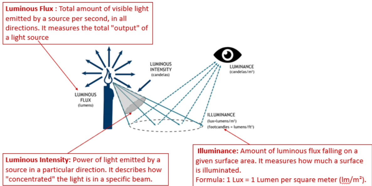
FIG.7 Photometric units
