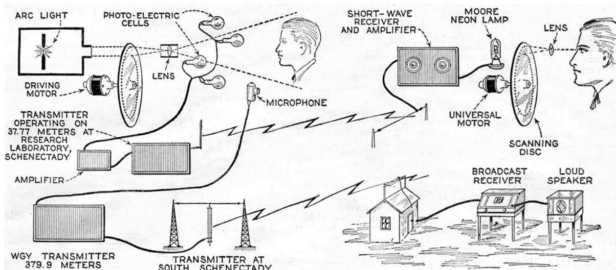
FIG.2 Transmission and Reception of Mechanical Television Signals
